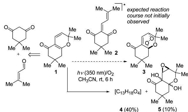
Scheme 2. Attempted Photooxygenation of 2 H -Pyrans 1
